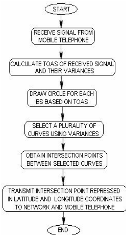
Flowchart showing the steps involved in locating a mobile telephone
