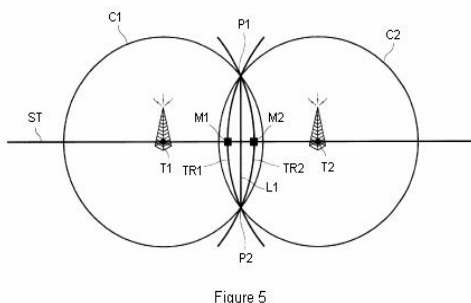
Figure3.5, illustrates a proposed method for mobile telephone location
